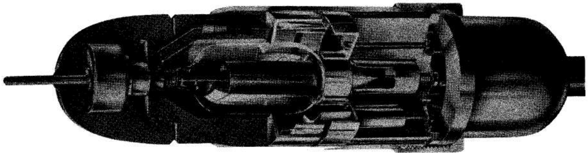
Figure 3-3. Cutaway View of High-Frequency Probe
