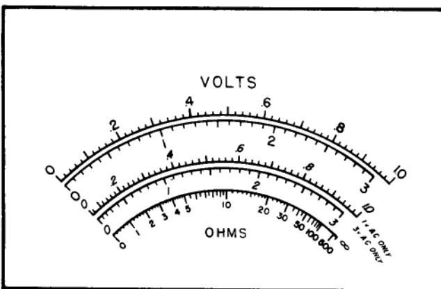
Figure 1-1. Meter Scale Calibration \Phi 410B
