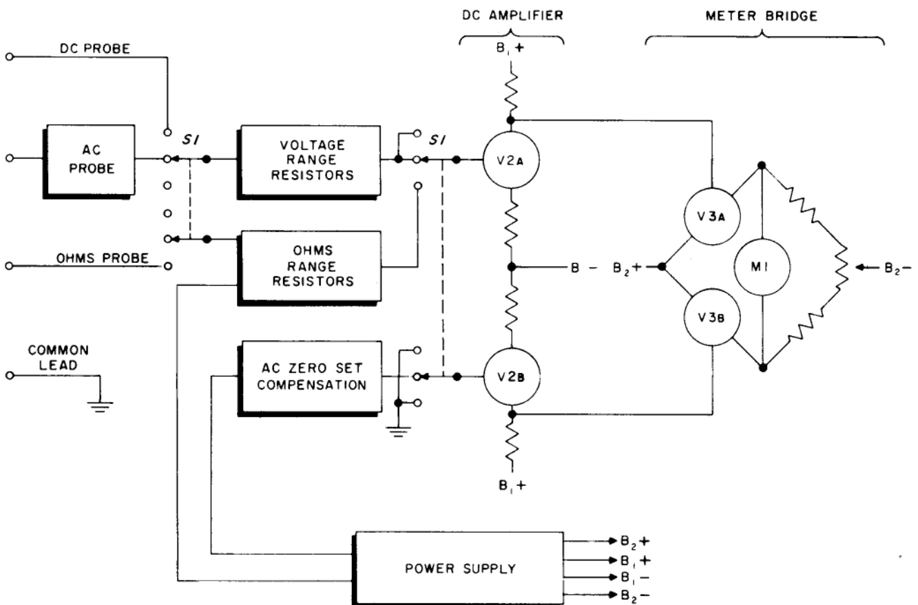
Figure 3-1. Block Diagram of \Phi Model 410B
