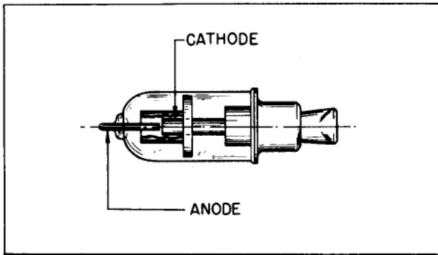
Figure 3-4. Actual Size Drawing of High-Frequency Diode
